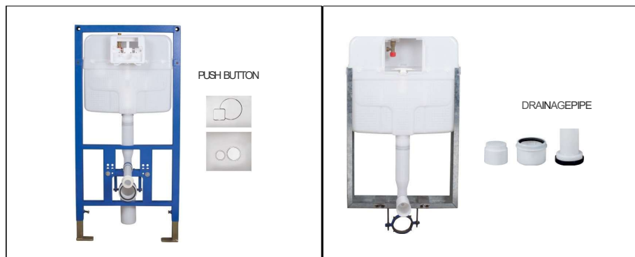
WCT-001 (Wall hung Concealed tank) Weight - 2.20Kg. L 590 B 75 D 1140
